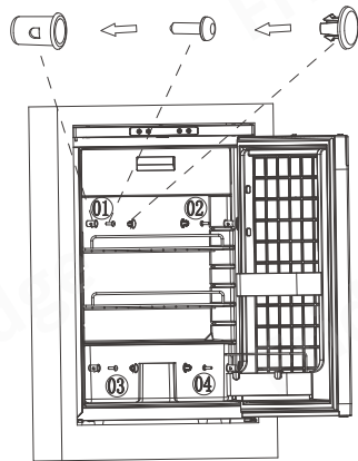
(Installation)
